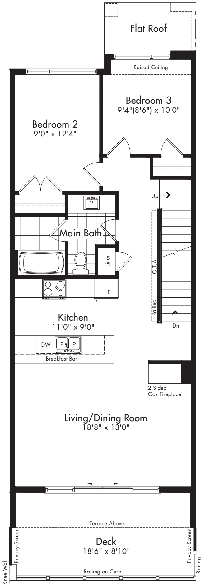
Second Floor - Elevation A
