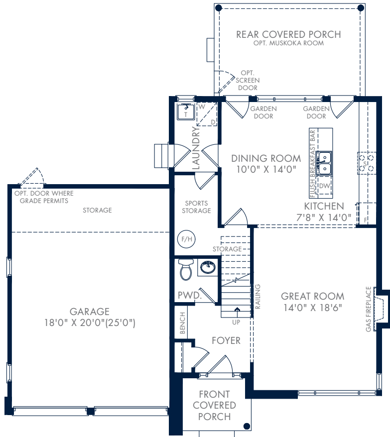
GROUND FLOOR – ELEVATION C 1,616 SQ.FT.
