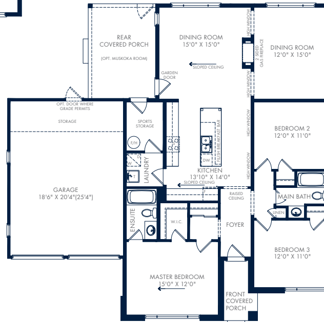
GROUND FLOOR – ELEVATION C
