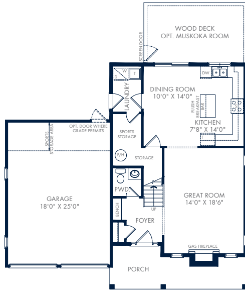
GROUND FLOOR – ELEVATION A
