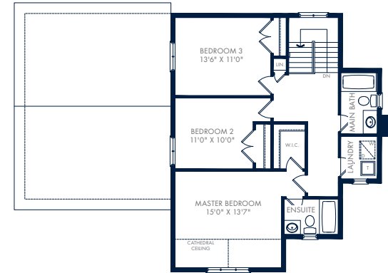
LOFT FLOOR – ELEVATION A
