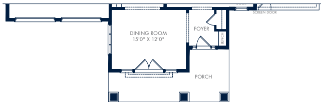
GROUND FLOOR – ELEVATION C
