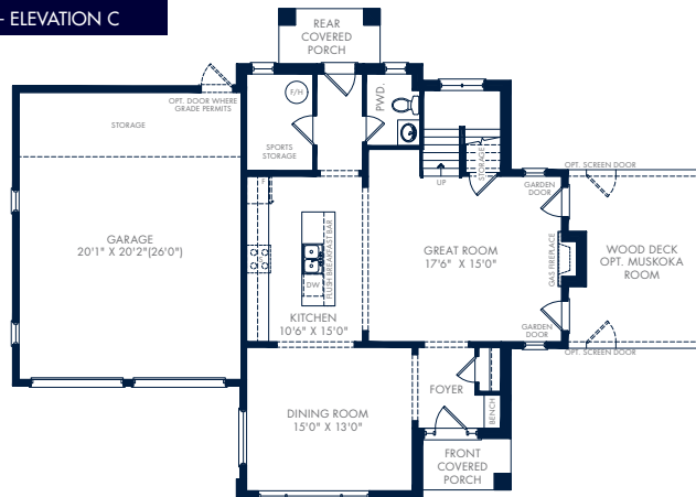
GROUND FLOOR – ELEVATION C
