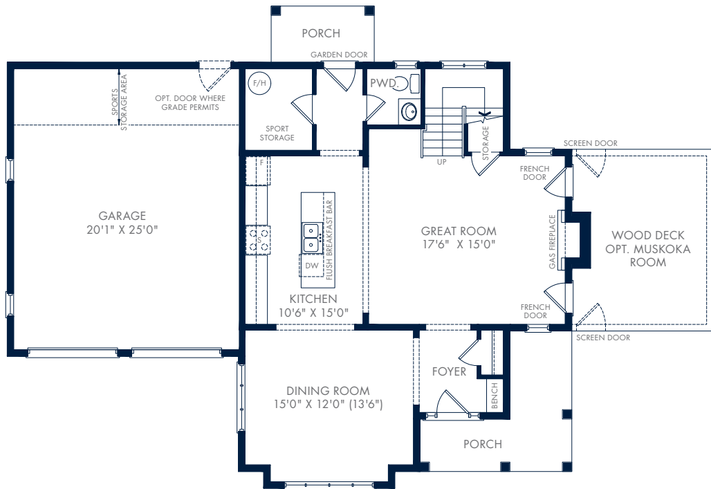
GROUND FLOOR – ELEVATION B
