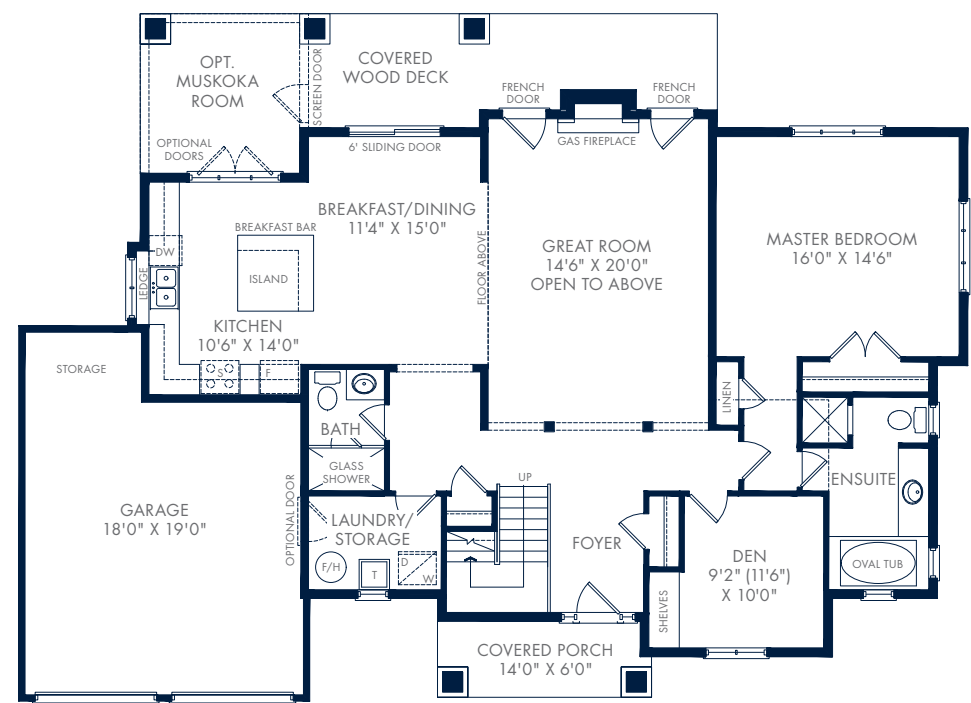
GROUND FLOOR – ELEVATION B REAR 2,183 SQ.FT.
