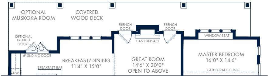
GROUND FLOOR – ELEVATION B REAR 2,183 SQ.FT.
