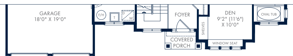
GROUND FLOOR – ELEVATION B FRONT
