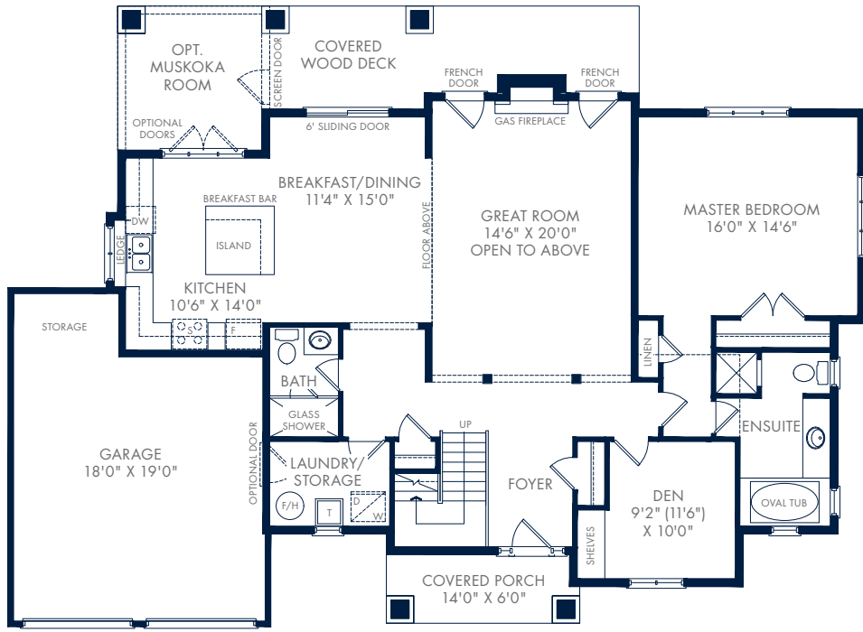
GROUND FLOOR – ELEVATION B REAR
