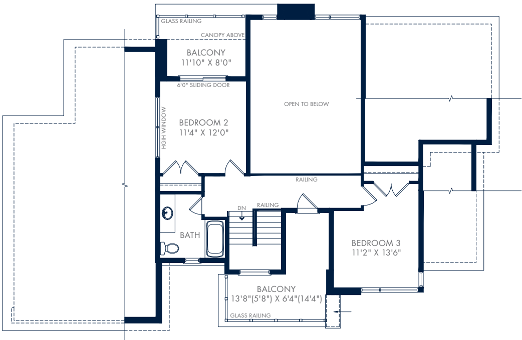
LOFT FLOOR – ELEVATION C
