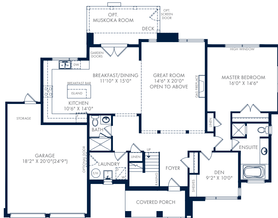
GROUND FLOOR – ELEVATION C
