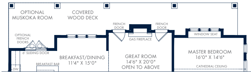
GROUND FLOOR – ELEVATION B REAR
